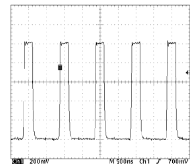
1MHz Frequency (Externally Triggered) 250ns Pulse Width, 10A Output
