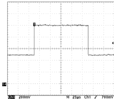
10A, 126µS Pulse On 5A Bias Current (Ground Indicated By "1" Marker)
