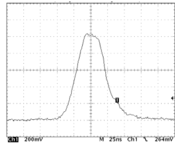
50ns Minimum Pulse Width, <30ns Rise And Fall Times, 10A Output
