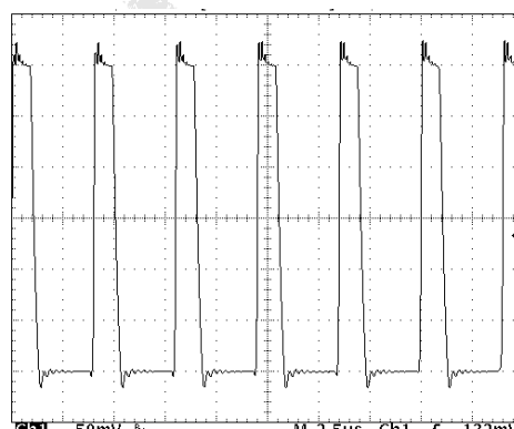
250KHz Frequency, 60A Output (2.5μs/Div horizontal scale, 10A/Div vertical scale)
