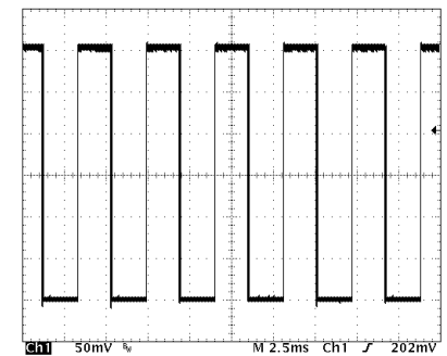
50% Duty Cycle, 2ms Pulse Width, 60A Output (2.5ms/Div horizontal scale, 10A/Div vertical scale)
