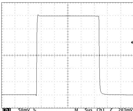
Typical Output Waveform 25μs Pulse Width, 60A Output (5μs/Div horizontal scale, 10A/Div vertical scale)
