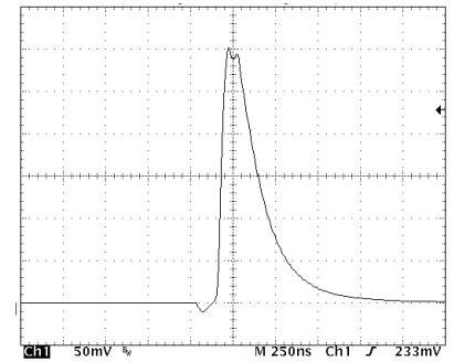
<50ns Rise Time, <400ns Fall Time, <250ns Pulse Width, 60A Output (250ns/Div horizontal scale, 10A/Div vertical scale)
